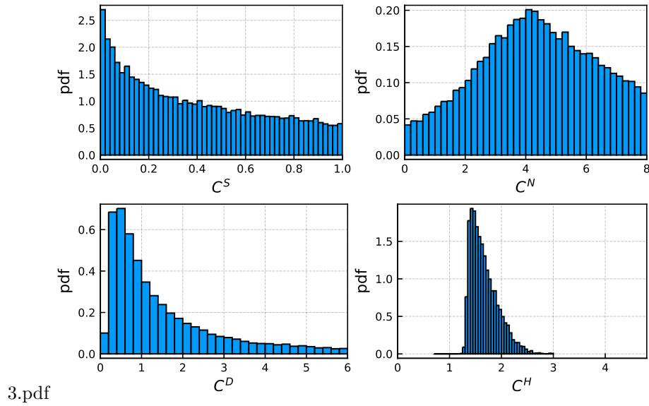
Figure 3. Parameter marginal posterior probability distributions. Marginal probability correspond to parameters parameters: C^S Surface Layer Fraction, C^N nonlocal diffusivity amplitude, C^D diffusivity amplitude, C^H mixing depth parameter. The probability distributions capture the notion of what parameter values are “good” and which ones are “bad”. For example, in the pdf for C^H we see that a value of 2.5 is probable but a value of 5 would be not be. This intuitively corresponds to saying that a value of 2.5 would be a “reasonable” choice whereas 5 would be “unreasonable”. The width of the C^S and C^N parameters suggest that KPP is quite insensitive to their values. A similar consequence holds for C^D , but there also seems to be a preference for values around one.
