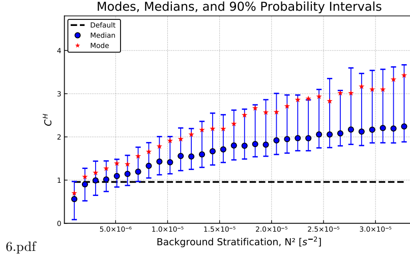
Figure 6. Mixing depth parameter optimized across various background stratification. The dots are the median values, the stars are the mode, and the error bars correspond to 90% probability intervals. The horizontal dashed line is the default value of the mixing depth parameter for reference. Here one can see that there mixing depth parameter when estimated across various regimes produces different results. This is a signature of a systematic bias in the parameterization.
